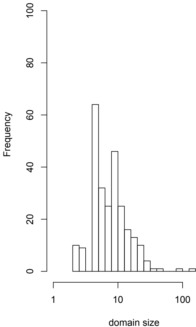
Histogram of the length of significant domains (log-scale) for the three state HMM
