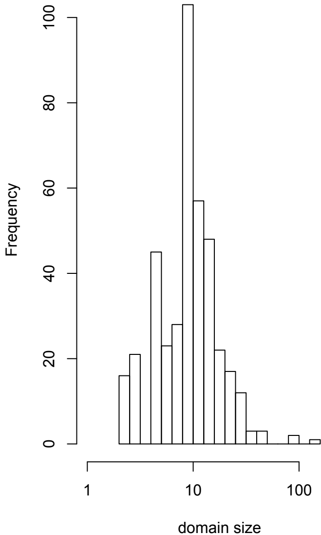
Histogram of the length of significant domains (log-scale) for the two state HMM
