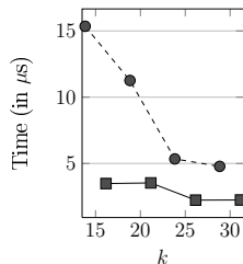
Query 1
