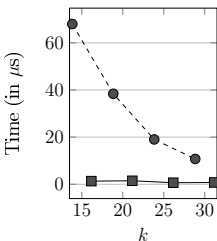
Query 3
