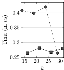
Query 4
