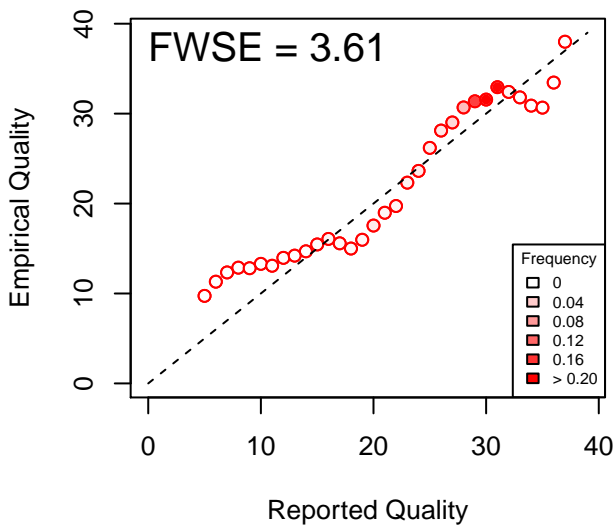
D Reported vs. Empirical Quality: After
