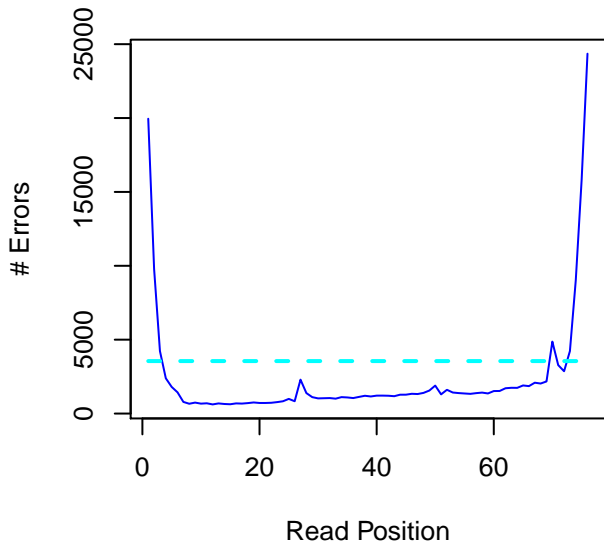
A Distribution of Errors by Read Position
