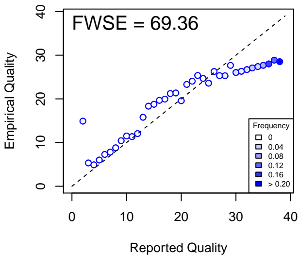
C Reported vs. Empirical Quality: Before
