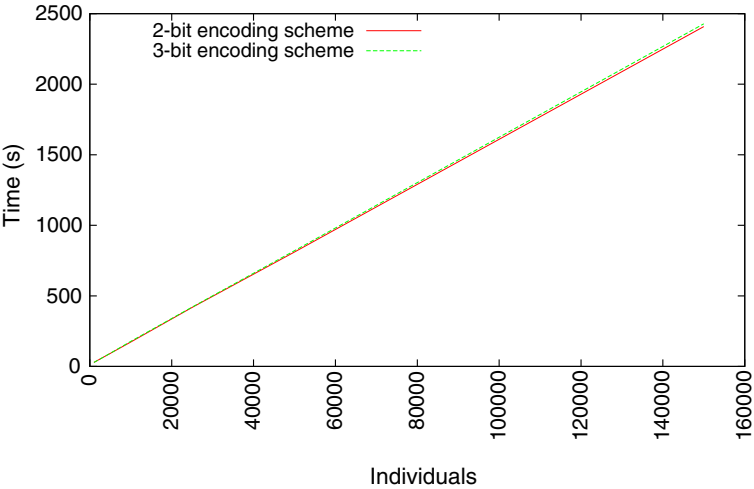
Epistasis (BOOST) algorithm Average runtime for 10000 Variants
