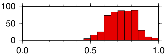
a Biological process
