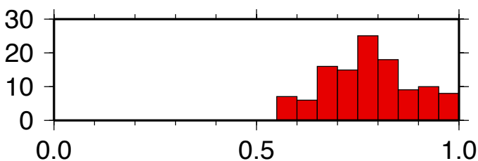
b Cellular component
