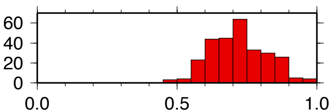
c Molecular function
