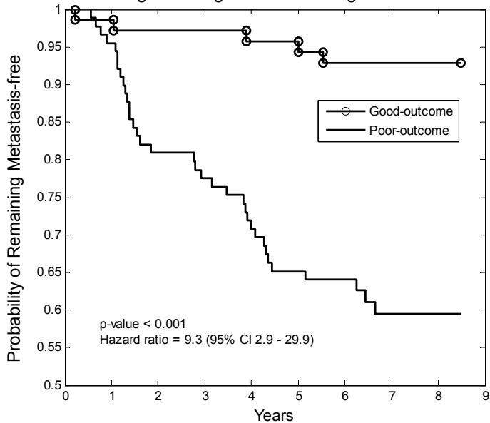
Prognostic Signature from Integrated Data
