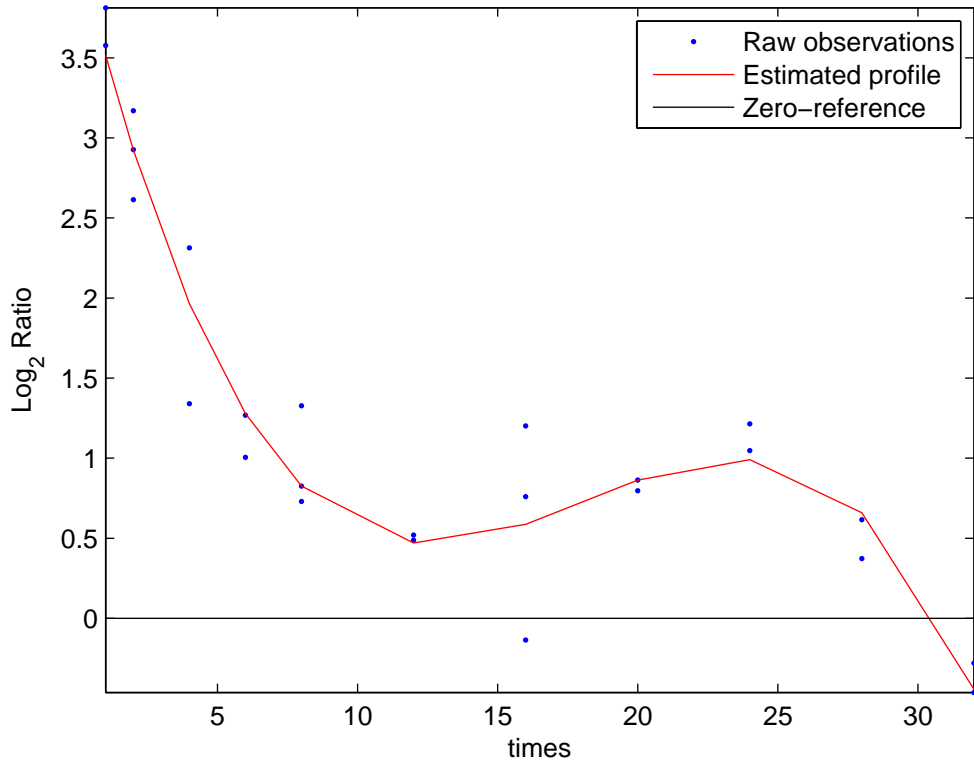
G7116 detected as differentially expressed in rank 2
