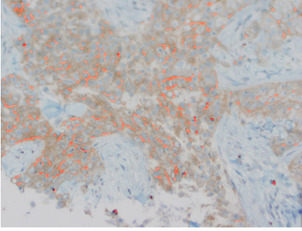
Threshold k = 15
