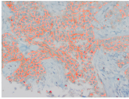
Threshold k = 5
