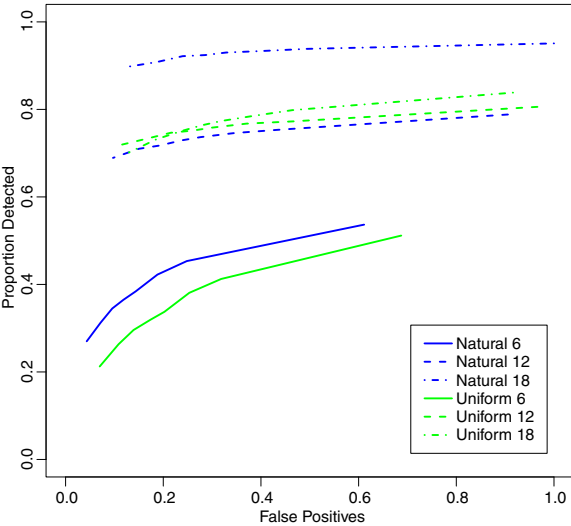
Pseudo-ROC of Outbreak Detection
