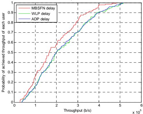
Empirical CDF
