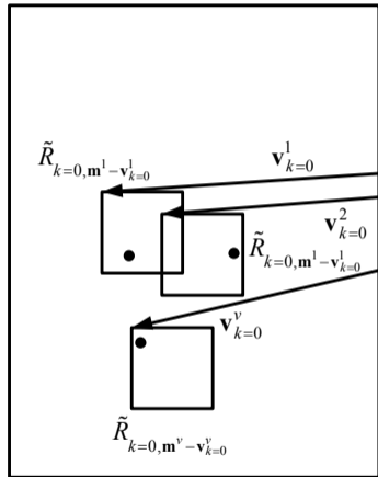
Preprocessed reference frame 0: \tilde{R}_{k=0}
