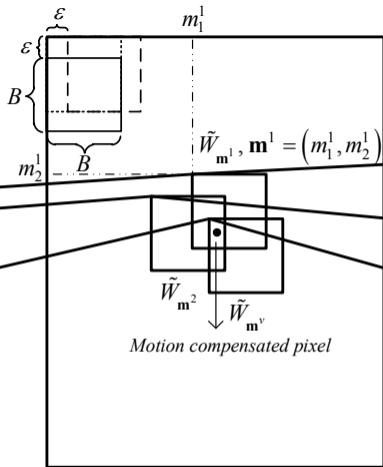
Decoded and upscaled hash frame: \tilde{W}
