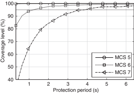
AL-FEC code rate = 0.6
