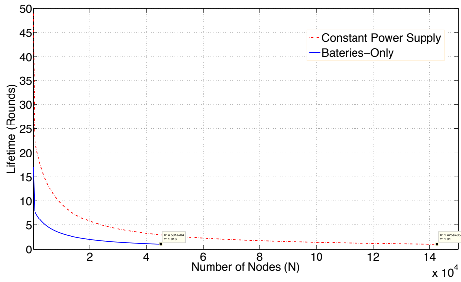
Fig. 12. System Lifetime for Different Number of Nodes in the Network.
