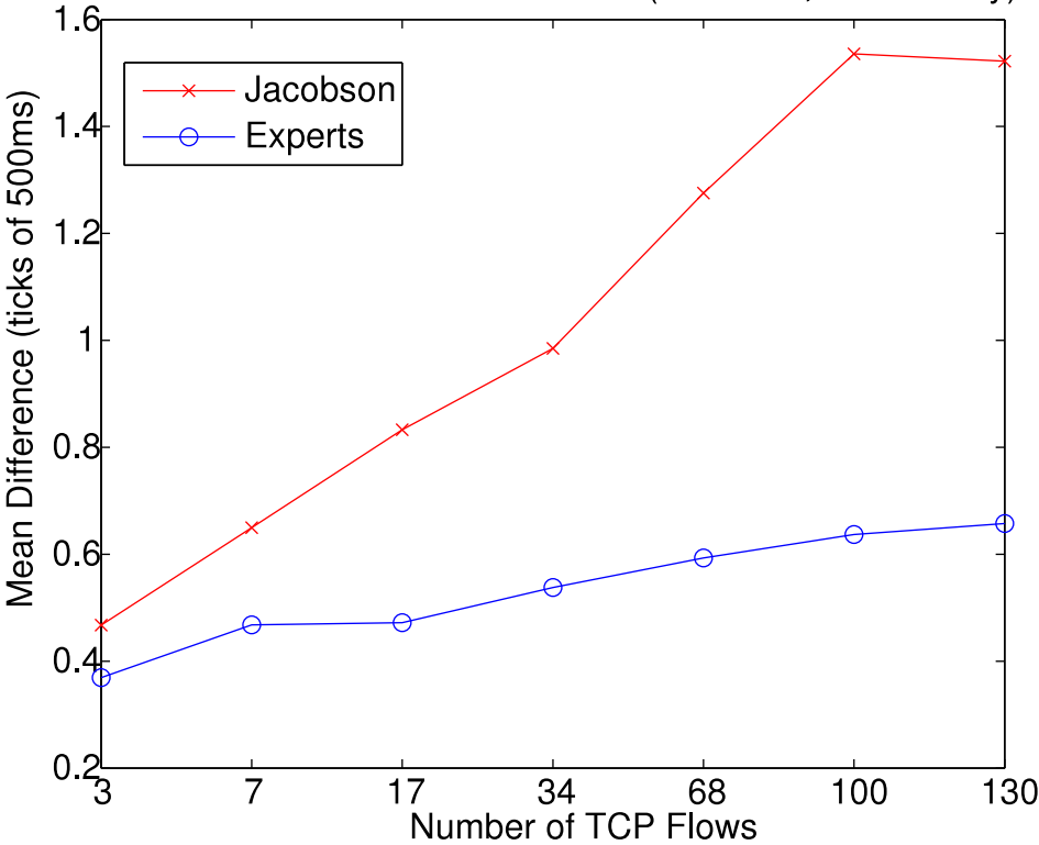
Mean Error on RTT Prediction (20 nodes, NO mobility)
