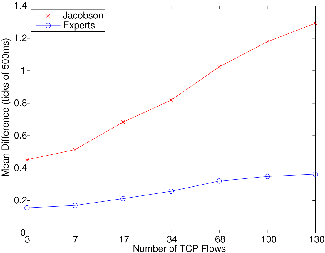
Mean Error on RTT Prediction.
