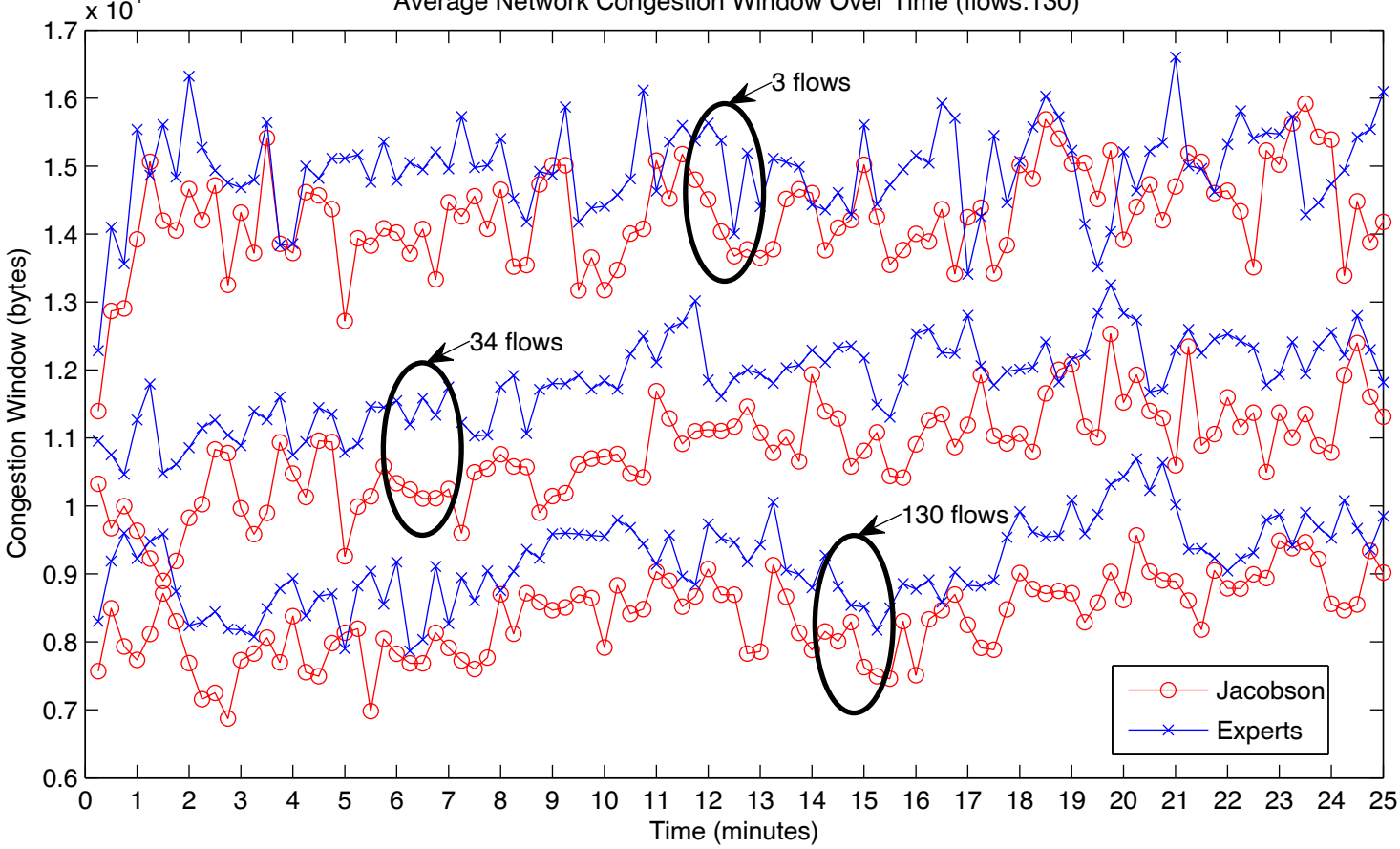
Average Network Congestion Window Over Time (flows:130)
