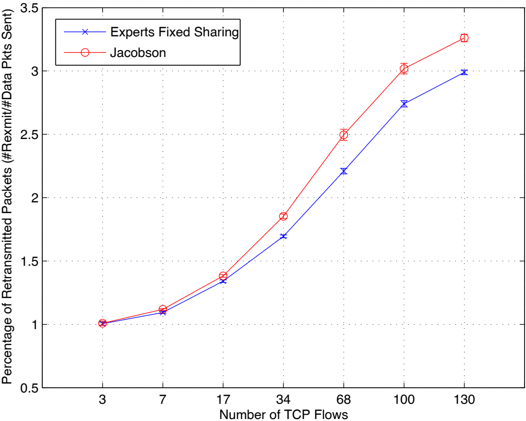
Percentage of Retransmitted Packets
