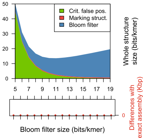
Probabilistic dBG and cFP structure
