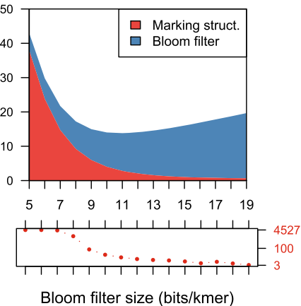
Probabilistic de Bruijn graph
