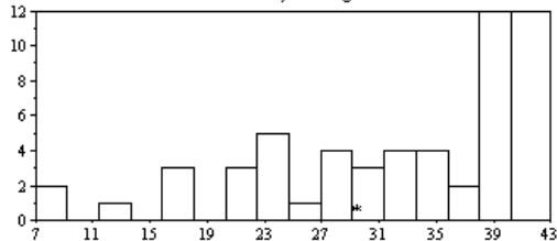
Comm. 2, clust. coeff.
