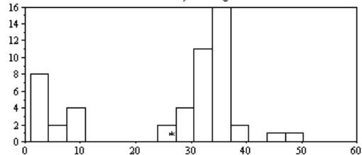
Comm. 1, clust. coeff.
