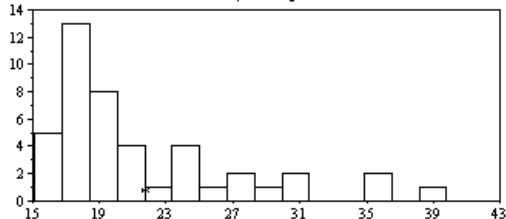
Comm. 2, match. ind.
