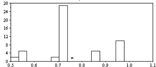
Comm. 1, av. sh. path. dist.
