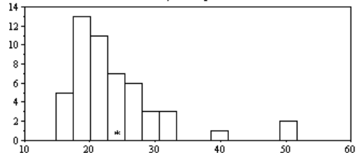
Comm. 1, match. ind.
