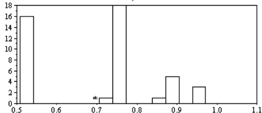
Comm. 2, av. sh. path. dist.
