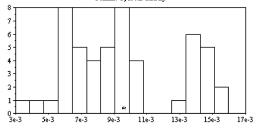
Comm. 1, coeff. var. near. dist.
