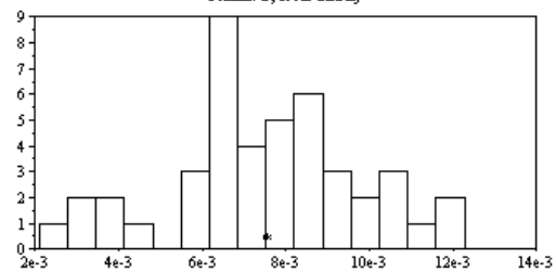
Comm. 2, coeff. var. near. dist.
