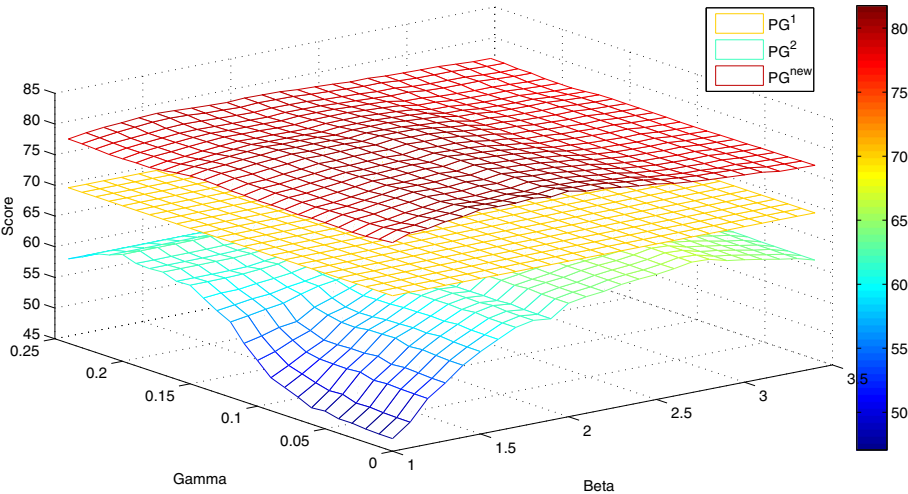
Comparison of perturbation graph performances
