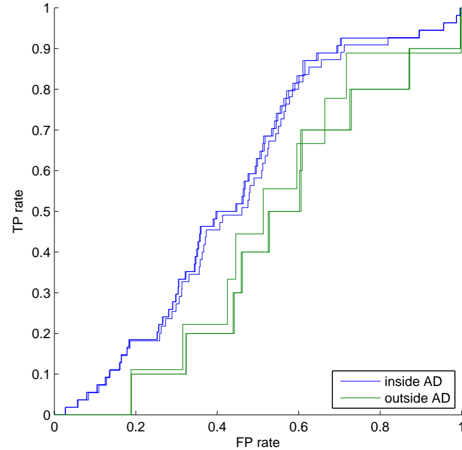
Marginalized Graph Kernel
