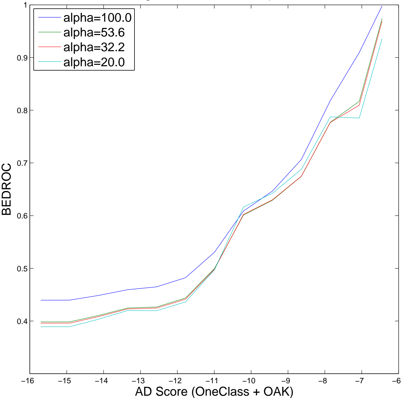
AD filtering effects on BEDROC performance
