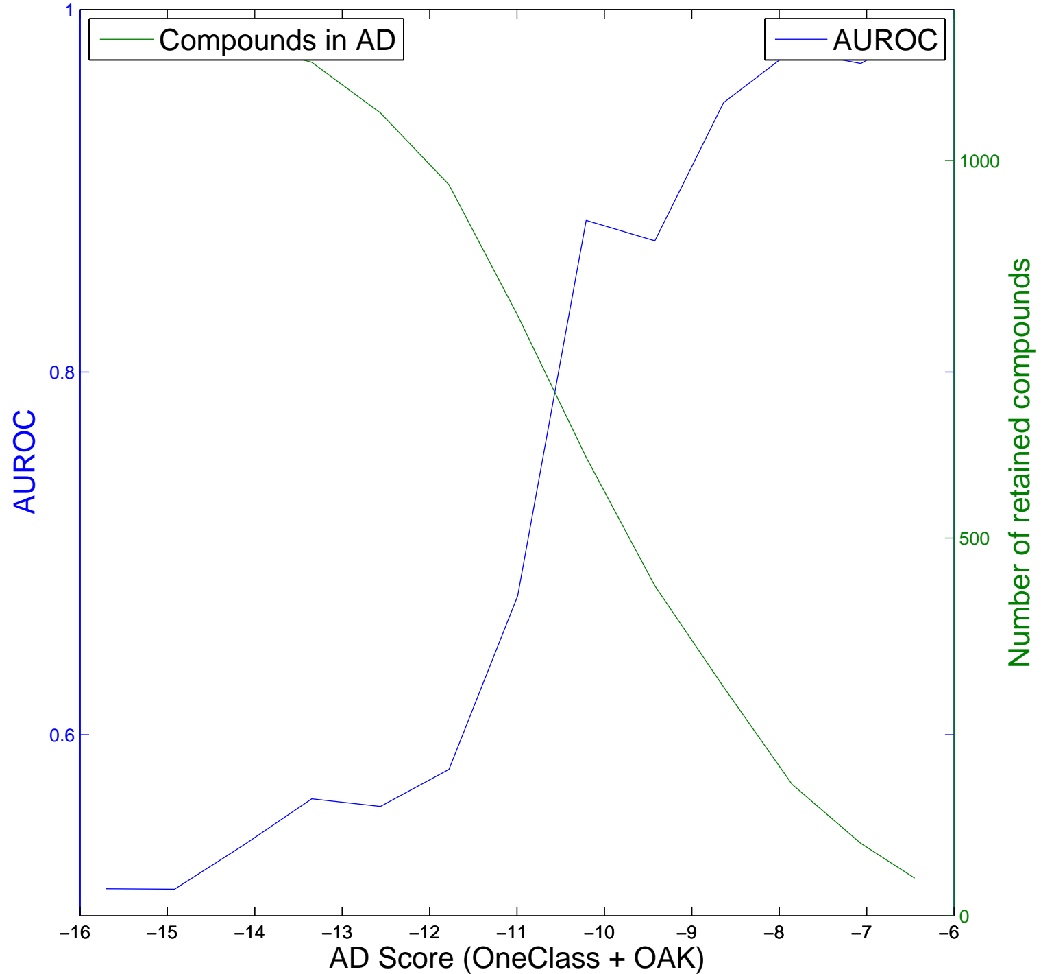
AD filtering effects on AUROC and compound count performance
