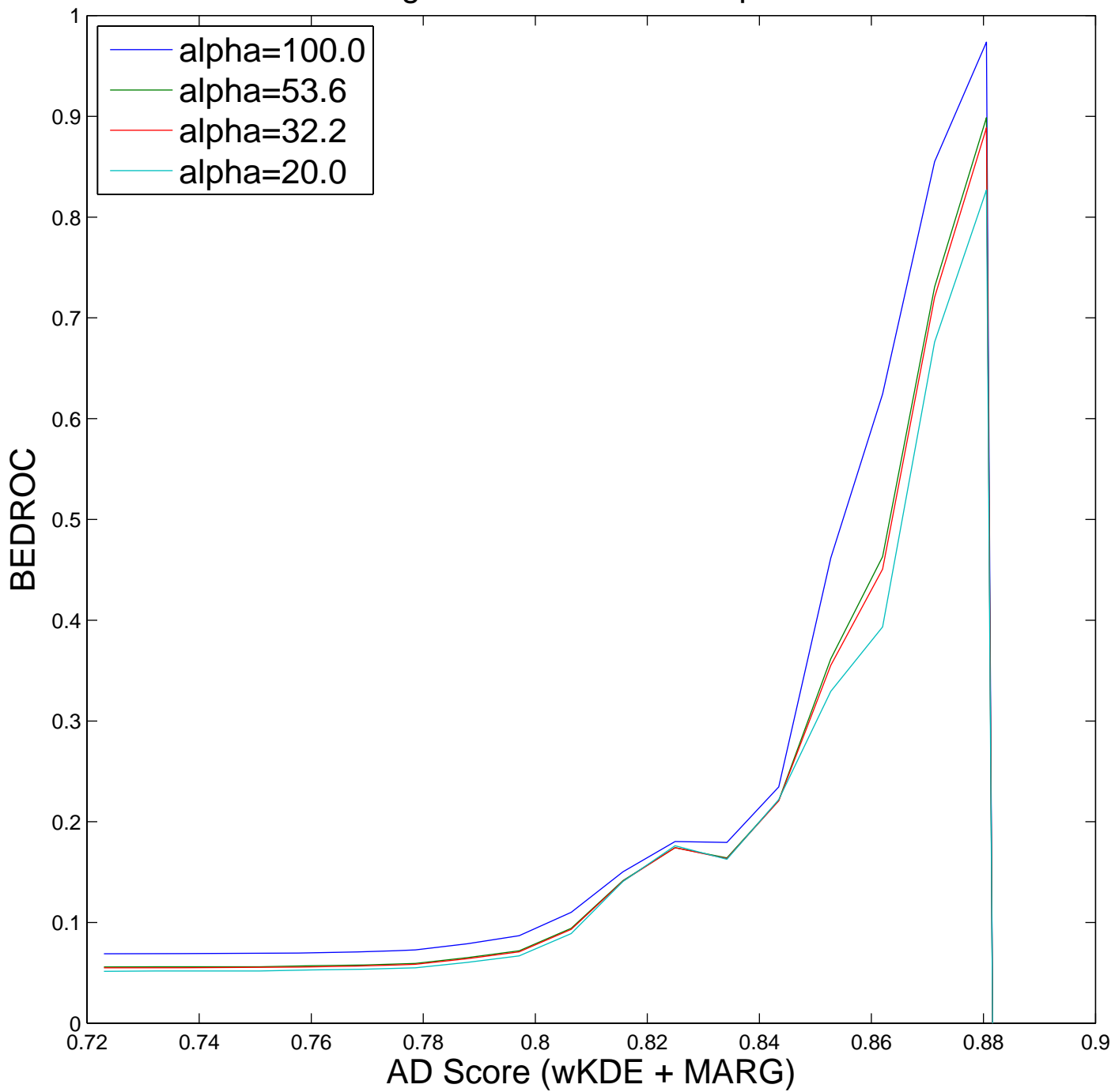
AD filtering effects on BEDROC performance
