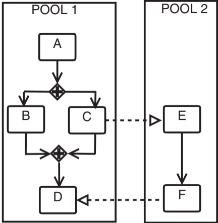
b) Multiple BPMN processes
