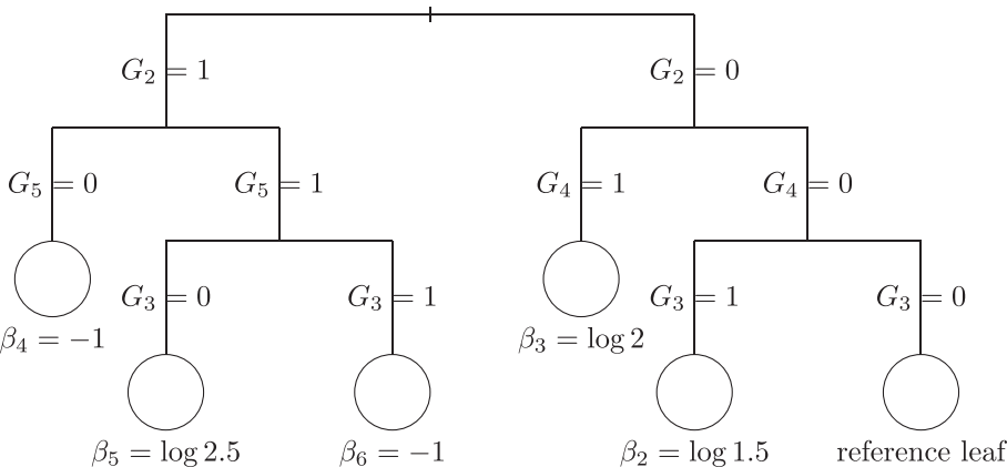
Simulated tree for scenario 3
