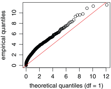
Trees with 5 leaves
