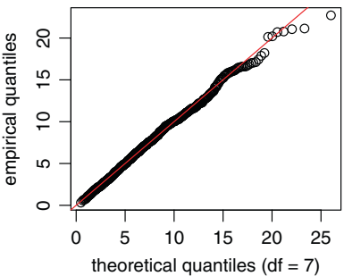
Trees with 8 leaves
