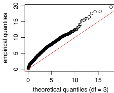
Trees with 7 leaves
