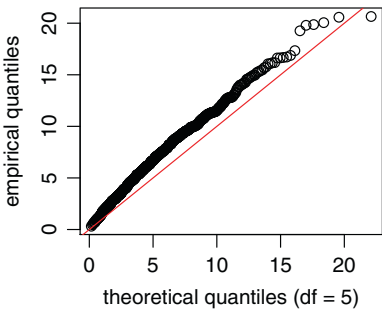
Trees with 6 leaves
