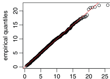
Trees with 6 leaves
