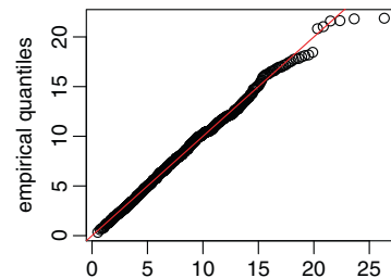
Trees with 7 leaves
