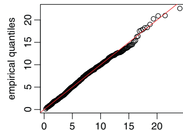
Trees with 4 leaves
