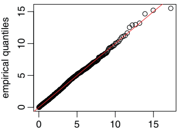
Trees with 2 leaves
