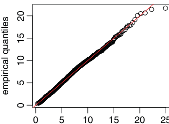
Trees with 5 leaves
