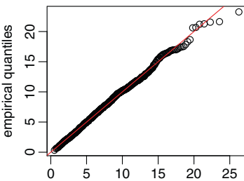
Trees with 8 leaves
