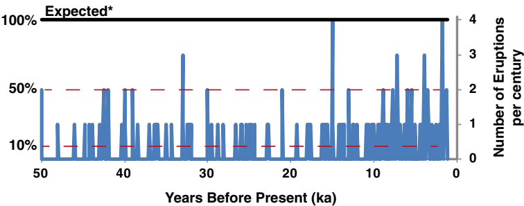
(c) M6-6.9
