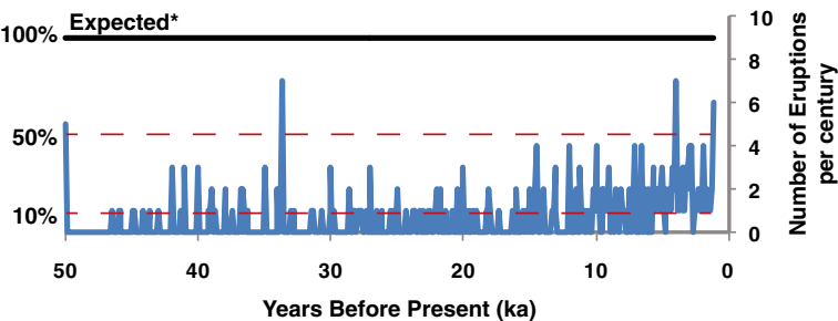
(c) M6-6.9
