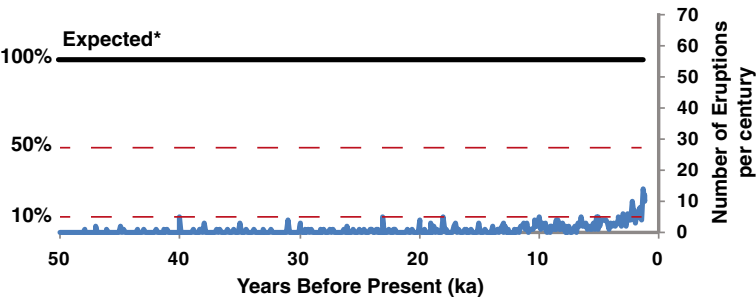
(a) M4-4.9
