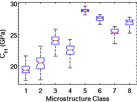
(a) Distribution of Modulus C_{11}
