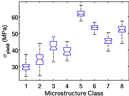
(b) Distribution of Yield Stress
