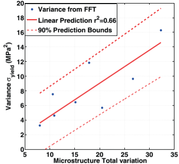
(b) Correlation of variance in yield strength with microstructure total variation
