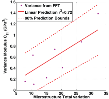
(a) Correlation of variance in C_{11} Modulus with microstructure total variation
