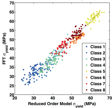
(b) Yield Stress Model Validation
