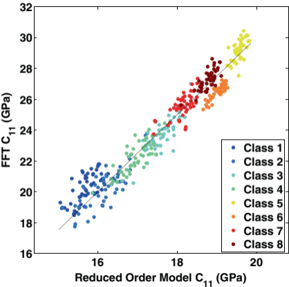
(a) Modulus C_{11} Model Validation
