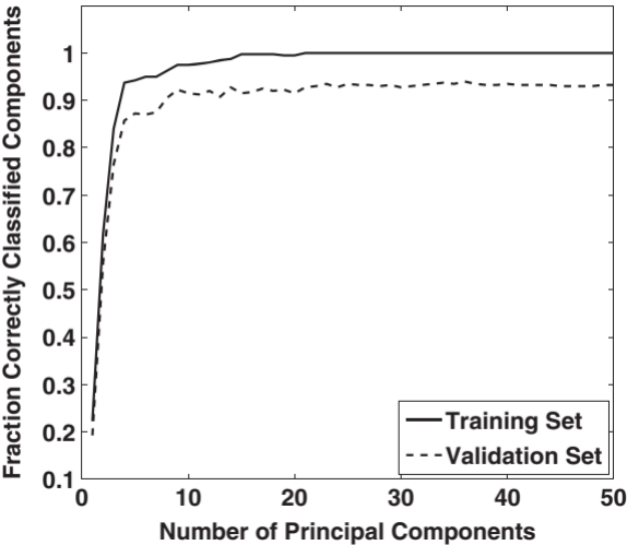
Accuracy of SVM Classification
