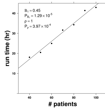
Figure 1 ISOpureR run times for the (A) Bhattacharjee dataset and the (B) Wang dataset. A comparison of run times for different number of transcripts, patients, and normals for the Bhattacharjee lung adenocarcinoma dataset and the Wang prostate cancer dataset. The full Bhattacharjee dataset contains 8383 transcripts, 139 patients, and 17 normal samples and the full Wang dataset contains 18185 transcripts, 109 patients, and 45 normal samples. For (i) the number of patients and normals remained the same as for the full datasets, and only the number of transcripts was changed. For (ii) only the number of patients was changed, and for (iii) only the number of normal samples was changed.
