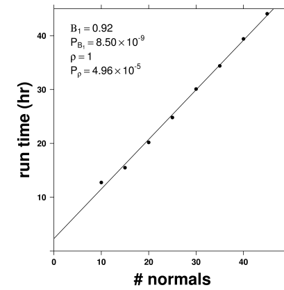
Figure 1 ISOpureR run times for the (A) Bhattacharjee dataset and the (B) Wang dataset. A comparison of run times for different number of transcripts, patients, and normals for the Bhattacharjee lung adenocarcinoma dataset and the Wang prostate cancer dataset. The full Bhattacharjee dataset contains 8383 transcripts, 139 patients, and 17 normal samples and the full Wang dataset contains 18185 transcripts, 109 patients, and 45 normal samples. For (i) the number of patients and normals remained the same as for the full datasets, and only the number of transcripts was changed. For (ii) only the number of patients was changed, and for (iii) only the number of normal samples was changed.
