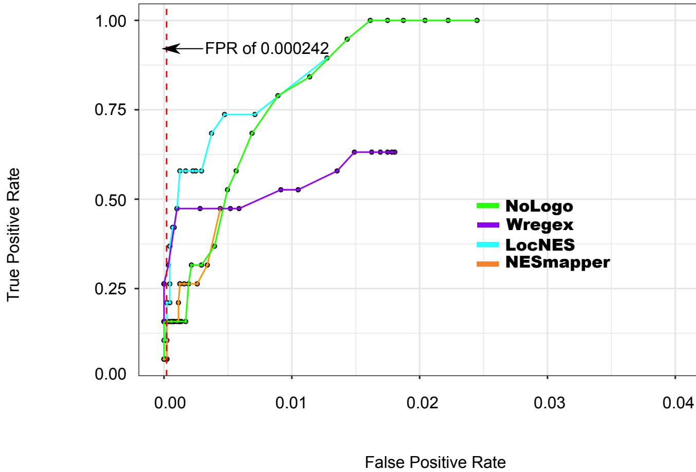
ROC curve NoLogo vs Wregex vs LocNES vs NESmapper
