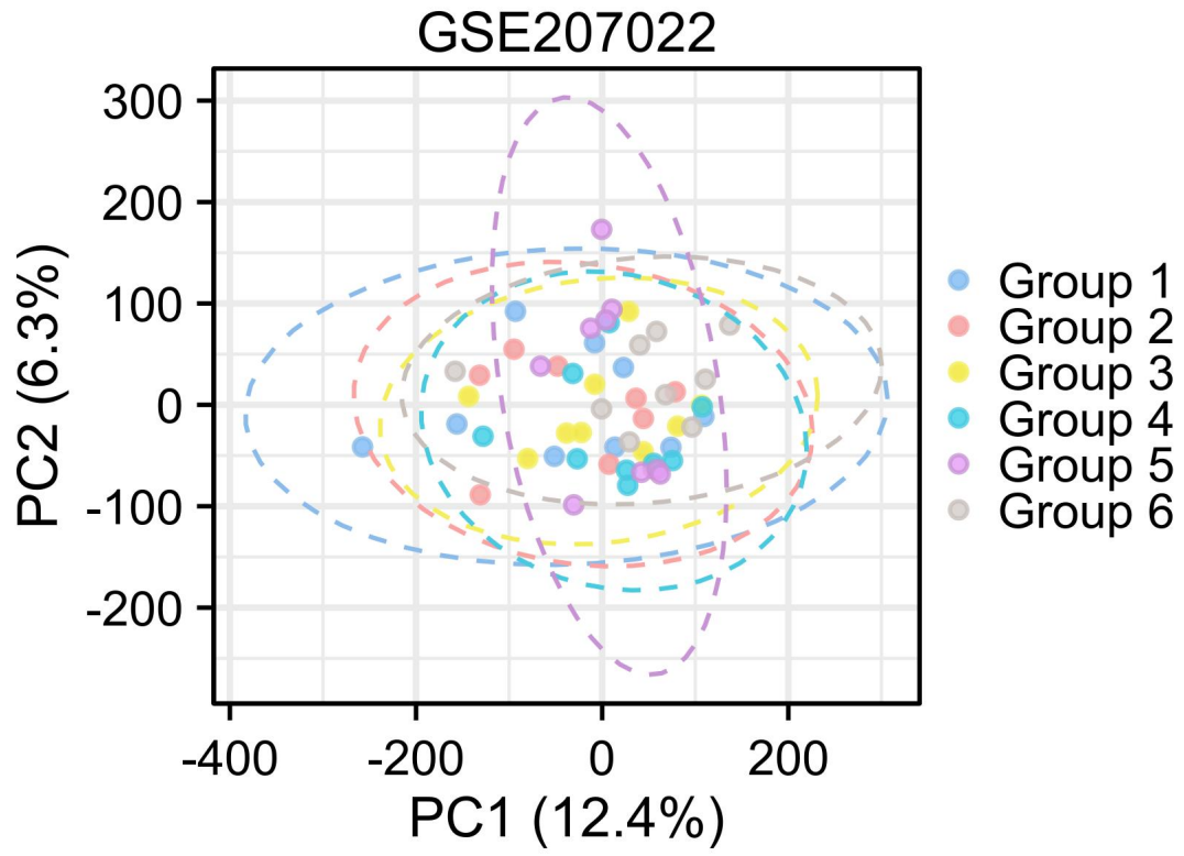
Figure S1. Principal component analysis (PCA) plot showing 54 samples in 6 groups.
