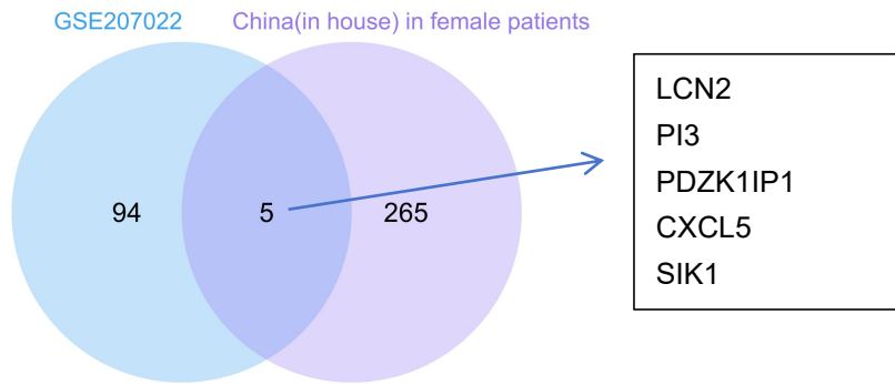
Figure S3. Venn diagrams of the differential genes between the discovery dataset and female samples (n = 6) of the validation dataset.
