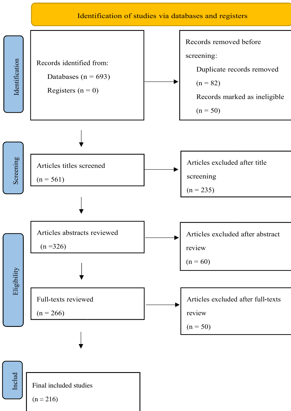
Fig. S1 PRISMA flowchart of the study selection process. The literature was conducted in accordance with the preferred reporting items for systematic reviews and meta-analysis (PRISMA) statement
