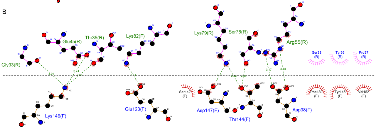
Fig. S3. (A) The 2D protein docking graph shows the interactive forces and distances between TLR1 and spike protein. (B) The 2D protein docking graph shows the interactive forces and distances between TNFSF4 and TNFRSF4.
