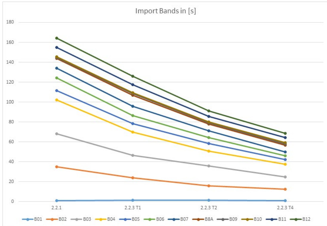
Figure 2: Performance improvement using OpenJPEG 2.3 and multithreading
