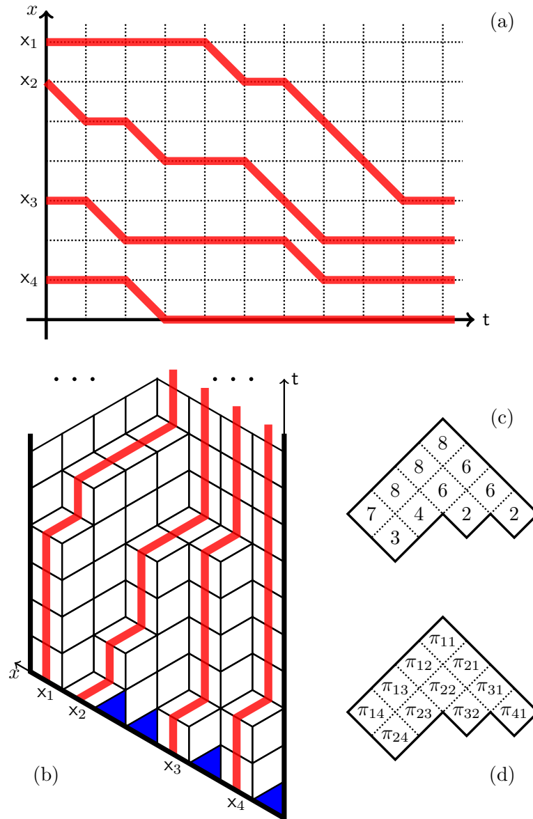
Figure 3. (a) A trajectory of the process \Upsilon_m with m = 4 and initial configuration \vec{x} = (7, 6, 3, 1) ; (b) A bijective interpretation of the trajectory as a lozenge tiling (the shaded triangles correspond to \mathbb{Z}_{\geq 0} \setminus \vec{x} and are removed from the strip); (c) The corresponding plane partition of shape (4, 4, 2, 1) = (7, 6, 3, 1) - (3, 2, 1, 0) ; (d) Encoding the elements of the plane partition which must satisfy \pi_{41} \geq 0 , \pi_{32} \geq 1 , \pi_{24} \geq 3 , and \pi_{14} \geq 3 .
