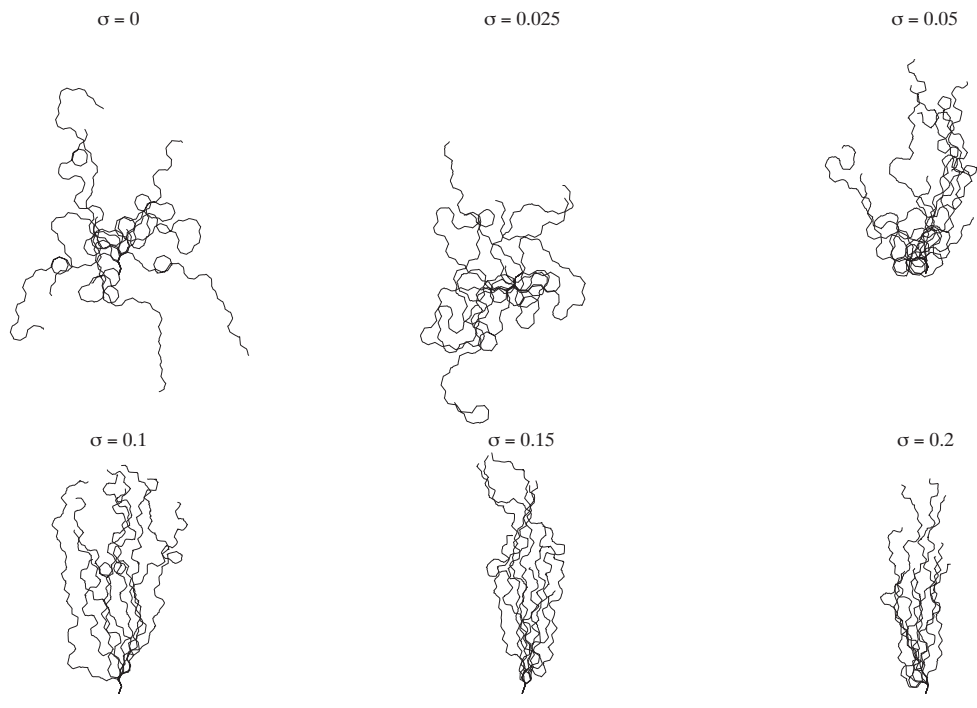
Figure 7: Trajectories of the centroids of cells migrating upwards in linear chemotactic gradients of varying strength.
