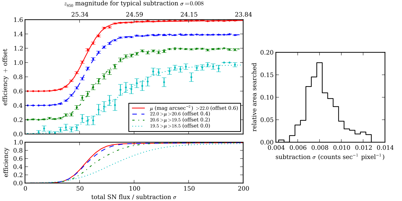
Figure 5. Point source detection efficiency in a single subtraction, as a function of the ratio of total point source flux to subtraction noise \sigma (counts \text{sec}^{-1} pixel ^{-1} ). The artificial point sources are split into four bins depending on the underlying galaxy surface brightness \mu (mag \text{arcsec}^{-2} ) at the point source position. The efficiency curve is calculated separately for each bin. In the upper left panel, the four bins are shown, offset for clarity. In the lower left panel, the fitted curves are reproduced without offset for comparison. Approximately 72,000 artificial point sources were used in total. The right panel shows the distribution of the noise level in the subtractions. The noise level differs by a factor of about two from the deepest to shallowest subtractions searched.
