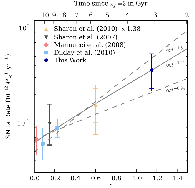
Figure 14. Cluster rate measurements (all galaxy types) from this work and the literature. The rate of Sharon et al. (2010) shown has been adjusted upward by 38% from the reported rate (see text). The top axis shows the time elapsed since an assumed cluster formation redshift of z_f = 3 . The solid grey line represents the SN Ia rate for the best-fit power-law DTD: \mathcal{R}_{\text{SN Ia}}(t) = \Psi(t)/m(t) , where \Psi(t) \propto t^s . The dotted grey lines show the range of 1\sigma error on s .
