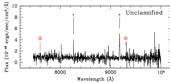
Fig. A.33. Above, a finding chart centered on SuF02-026 and below, the spectrum. This candidate has two unidentified emission lines with differing line profiles and spatial morphologies. The line at \sim 8300 \text{ \AA} is unresolved while the line at \sim 9200 \text{ \AA} is spatially and kinematically resolved into three components. This candidate was photometrically monitored and it has a supernova-like light curve.
