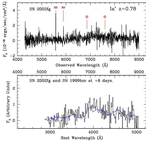
Fig. A.16. Above, a finding chart centered on SN 2002fg (S02-075), a SN Ia* at z = 0.78 , and below, the spectrum. Since the Si II feature at 4000 \text{ \AA} is not clearly detected in this candidate and since there are no spectral features from the host, the classification and the redshift are derived from the fit. The candidate was observed several weeks after it was discovered, so it is likely that the spectrum was taken past maximum light. The best matching nearby SN Ia is SN 1999bm at 6 days past maximum light. The signal-to-noise ratio is also relatively low and the SiII feature at 4000 \text{ \AA} is not detected, so the classification is qualified with an asterisk.
