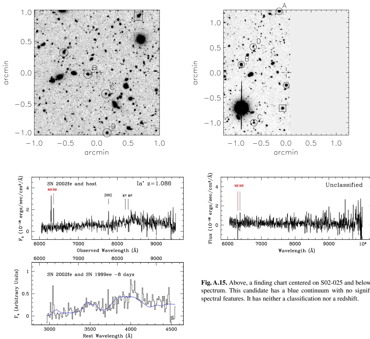
Fig. A.14. Above, a finding chart centered on SN 2002fe (S02-002), a SN Ia* at z = 1.086 , and below, the spectrum. The profile of the line that we have identified as [OII] is affected by a nearby bright night sky line; however, the line is clearly detected in the 2-dimensional spectrum. This line, together with the probable detection of the H and K Ca II lines in the host, enables us to measure a secure redshift. The signal-to-noise ratio of the spectrum is relatively low and the Si II feature at 4000 Å is not detected, so the classification is qualified with an asterisk. In some nearby SNe Ia that are observed one to two weeks before maximum light, the Si II feature is absent. The best fit nearby SN Ia, SN 1999ee, shows no Si II at 4000 Å.
