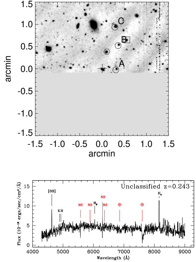
Fig. A.21. Above, a finding chart centered on C02-034, an unclassified candidate at z = 0.243 , and below, the spectrum. The host galaxy has emission lines in H α , H β and [OII]. The Calcium H and K absorption lines are also visible.
