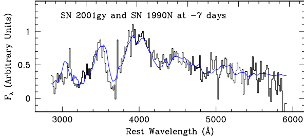
Fig. A.8. Above, a finding chart centered on SN 2001gy (S01-036), a SN Ia at z = 0.511 , and below, the spectrum. The Si II feature at 4000 \text{ \AA} is clearly detected.
