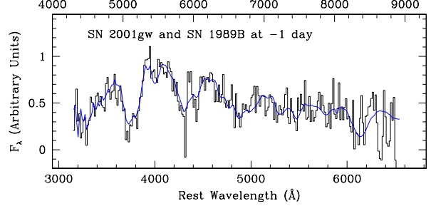
Fig. A.7. Above, a finding chart centered on SN 2001gw (S01-033), a SN Ia at z = 0.363 , and below, the spectrum. In addition to the Si II feature at 4000 \text{ \AA} , the Si II at 6150 \text{ \AA} is also visible. The redshift is derived from an [OII] emission line in the spectrum of the host galaxy (not shown here).
