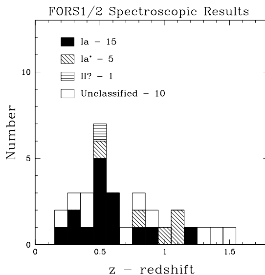
Fig. 2. A redshift histogram of the candidates.
