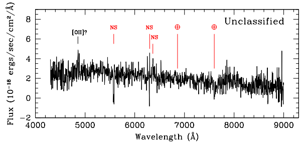
Fig. A.17. Above, a finding chart centered on SN 2002fr (C02-016), an unclassified candidate that might be at z = 0.303 , and below, the spectrum. This candidate has a very well sampled light curve (7 points), which shows a dramatic rise over the first 5 days. The spectrum is dominated by slightly irregular blue continuum and there is a very weak line which would put the host at z = 0.303 if the line is identified as [OII].
