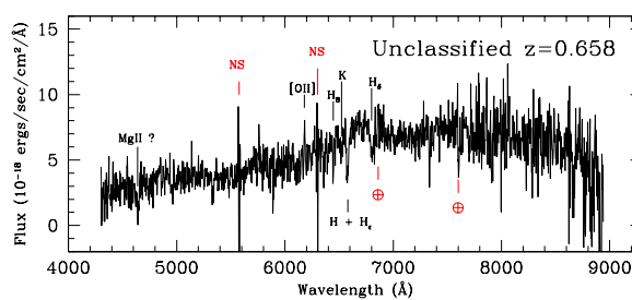
Fig. A.5. Above, a finding chart centered on SN 2001gs (S01-028), an unclassified candidate at z = 0.658 , and below, the spectrum. This is a faint candidate on a bright host that was observed during a period of relatively poor seeing. The percentage increase in the flux was only 27%, so most of the light in the spectrum is from the host, which has several Balmer absorption lines.
