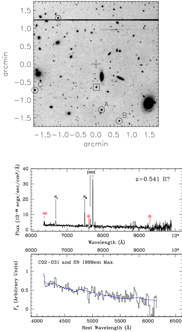
Fig. A.20. Above, a finding chart centered on C02-031, a possible Type II supernova at z = 0.541 and below, the spectrum. The host galaxy has emission lines in [OIII], H β and H γ . The tentative classification is based on the blue continuum and a weak H-beta line with a P-Cygni profile.
