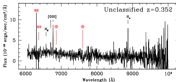
Fig. A.19. Above, a finding chart centered on SN 2002fp (C02-030), an unclassified candidate at z = 0.352 , and below, the spectrum. The host galaxy has emission lines in [OIII] and H_{\beta} . The continuum is blue and, at this signal-to-noise ratio, featureless. This candidate might be a SN II, since the pre-maximum spectra of SNe II are generally featureless and blue; however, without clear features in the continuum, we cannot assign a classification.
