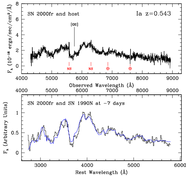
Fig. 3. A spectrum of SN 2000fr, a SN Ia at z = 0.543 with unambiguous detection of Si II at 4000 \text{ \AA} . In the upper spectrum, the un-binned spectrum of the candidate is plotted in the observer’s frame and is uncorrected for host galaxy light. Night sky subtraction residuals are marked with the letters “NS” and telluric absorption features are marked with the symbol \oplus . In the lower spectrum, contamination from the host is removed and the spectrum is rescaled and rebinned by 20 \text{ \AA} . This spectrum is plotted in black and it is plotted in both the rest frame (lower axis) and the observer’s frame (upper axis). For comparison, the best fitting nearby supernova is plotted in blue. SN 2000fr was first identified as a SN Ia in a very early spectrum that was taken with LRIS on the KeckII telescope on 2001 May 4th and was subsequently observed again with FORS1. The FORS1 spectrum has one of the highest S/N ratios of all securely identified supernovae in this paper. SN 2000fr was followed in the J-band with ISAAC 2004 and in the R- and I-bands with HST and ground-based telescopes (Knop et al. 2003). The J-band observations, which corresponds to the rest-frame I-band, show a clear second maximum about 30 days after the first maximum. A spectrum of the host galaxy (not shown here) shows emission in [OII] and [OIII] as well as Balmer absorption lines.
