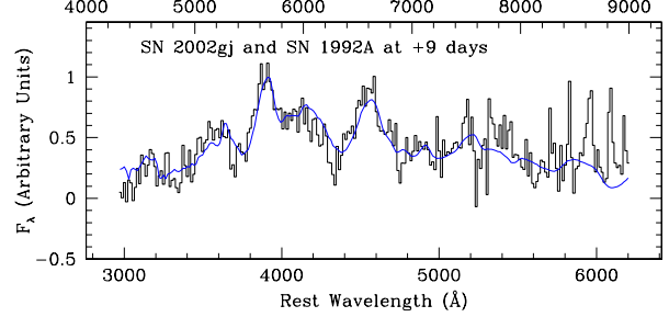
Fig. A.23. Above, a finding chart centered on SN 2002gj (T02-028), a SN Ia* at z = 0.45 , and below, the spectrum. From the spectrum alone, this candidate can be matched with either a SN Ia at 10 days after maximum light or with a SN Ic near maximum light, so the classification is qualified with an asterisk. The time of maximum that is derived from the light curve shows that the spectrum was taken about 10 rest frame days after maximum light, so the the candidate is very likely to be a SN Ia.
