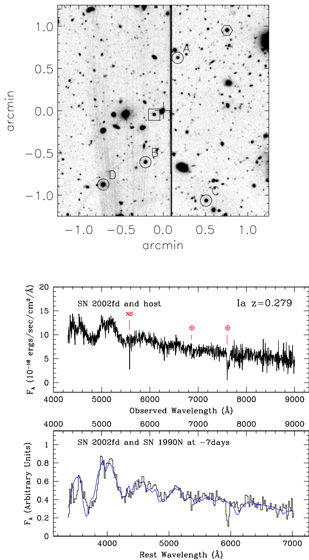
Fig. A.12. Above, a finding chart centered on SN 2002fd (S02-000), a SN Ia at z = 0.279 , and below, the spectrum. The Si II feature at 4000 \text{ \AA} is clearly detected, but the Si II feature at 6150 \text{ \AA} is relatively weak.
