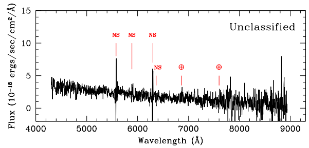
Fig. A.9. Above, a finding chart centered on S01-037, and below, the spectrum. Neither the classification nor the redshift of this candidate is known. The spectrum shows a strong blue continuum which is characteristic of Type II supernovae before maximum light; however, with neither a redshift nor clear spectral features, a classification cannot be made. The candidate was detected on search images that were taken on different dates and is stationary, so it is not an asteroid nor an artifact.
