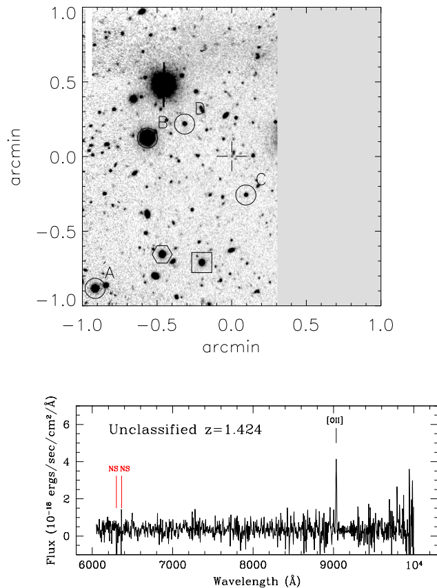
Fig. A.13. Above, a finding chart centered on S02-001, an unclassified candidate at z = 1.424 , and below, the spectrum. A single strong line and a featureless continuum. Given the width and shape of the line and the lack of other lines in the wavelength range covered by the spectra, the line is identified as the [OII] doublet at 3727 \text{ \AA} . It is unlikely that the line is \text{Ly}\alpha at z > 5 because the characteristic asymmetry of \text{Ly}\alpha in galaxies at z > 5 (Stern et al. 2000) and the jump in the continuum across the line are not evident in these spectra. Nor is the line likely to be \text{H}\alpha , as neither \text{H}\beta nor [OIII] are detected. The equivalent width of the line is greater than 50 \text{ \AA} so the host galaxy would be classified as an emission line galaxy (ELG) if the line were \text{H}\alpha (Kniazev et al. 2004). In ELGs, \text{H}\beta is typically three times weaker than \text{H}\alpha and the strengths of [OIII] and \text{H}\alpha are roughly equivalent. Given the strength of the detected line in these spectra, both [OIII] and \text{H}\beta should have been detected if the line was \text{H}\alpha .
