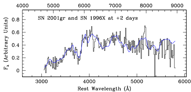
Fig. A.4. Above, a finding chart centered on SN 2001gr (S01-017), a SN Ia at z = 0.540 , and below, the spectrum. Although Si II feature at 4000 \text{ \AA} is not clearly detected in this candidate, the data are significantly better fit with SN Ia spectra than with the spectra of other types.
