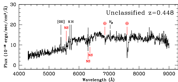
Fig. A.18. Above, a finding chart centered on SN 2002fm (C02-028), an unclassified candidate at z = 0.448 , and below, the spectrum. The percentage increase in this candidate was very small, only 13%, and the spectrum is dominated by the light from the host galaxy. However, there is excess flux at 6600 \text{ \AA} and 5600 \text{ \AA} that might be from a supernova. Unfortunately, an acceptable fit with a nearby SN Ia was not possible. In such cases, the fit depends critically on how well the galaxy template matches the spectrum of the host galaxy. Relatively small errors can leave significant residuals which can make the matching difficult. The most secure way of fitting this candidate will be take a spectrum of the host after the supernova has faded. The candidate is offset from the center of the host and the light curve is well sampled with four points before maximum light and four points after maximum light.
