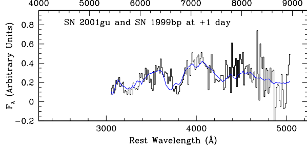
Fig. A.6. Above, a finding chart centered on SN 2001gu (S01-031), a SN Ia at z = 0.777 , and below, the spectrum. The host shows CaII H and K absorption lines and no detectable [OII] emission which suggests an early-type host. Since the Si II feature at 4000 \text{ \AA} is weak and contaminated by the H and K lines of the host, the classification is based on the fit. The redshift of the fit was constrained to that of the host. The wavelength coverage of the best matching nearby SN Ia, SN 1999bp, is restricted to rest frame wavelengths that are greater than 3000 \text{ \AA} , so the comparison is limited to these wavelengths.
