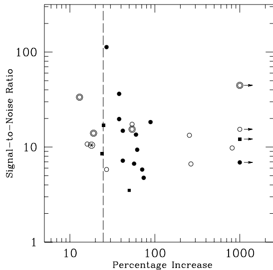
Fig. 4. The percentage increase versus the signal-to-noise ratio for candidates that were brighter than I = 24.7 at the time of discovery. Candidates that were classified as Ia ( Ia^* ) are plotted with solid circles (squares), C02-031 - a possible SN II - is plotted as a star and unclassified candidates are plotted with open circles. Candidates from the CFHT 2002 search are highlighted with large circles. Candidates with arrows have percentage increases that are greater than 1000%, which means that the host was considerably fainter than the candidate and perhaps undetected. The dashed line marks the region where the percentage increase is 25% or less. Candidates in this region are difficult to classify spectrally.
