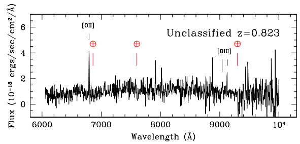
Fig. A.27. Above, a finding chart centered on SN 2002kq (SuF02-002), an unclassified candidate at z = 0.823 , and below, the spectrum. This candidate was photometrically monitored and it has a supernova-like light curve.
