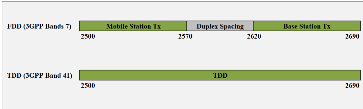
Figure 3. 2.5 GHz band plans
