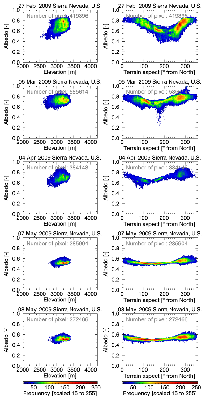
Figure 12. Snow albedo with respect to terrain elevation (left panels) and terrain aspect (right panels) in the Sierra Nevada in spring 2009.
