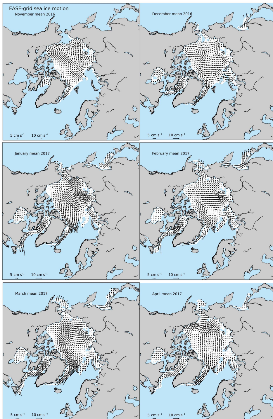
Figure 8. Mean monthly sea ice motion from the NSIDC Polar Pathfinder Data Set. Preliminary data provided by Scott Stewart, NSIDC.
