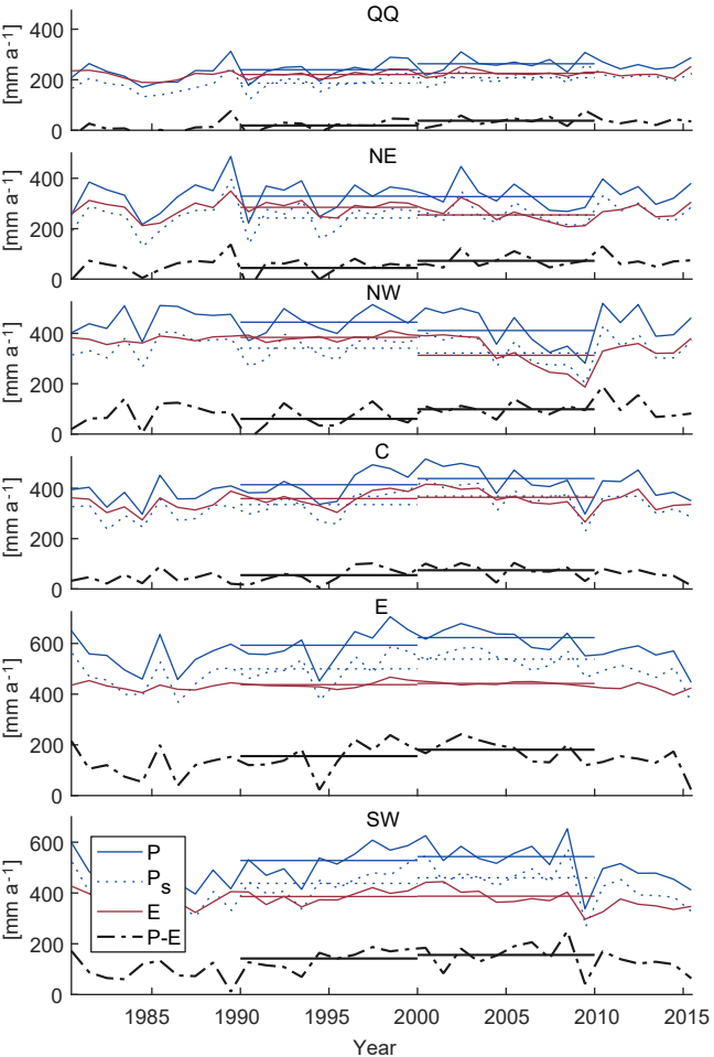
(a) ERA-Interim
