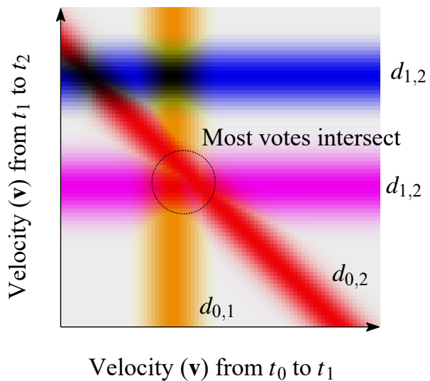
(a) Two-dimensional fuzzy Hough space
