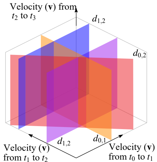
(b) Three-dimensional Hough space
