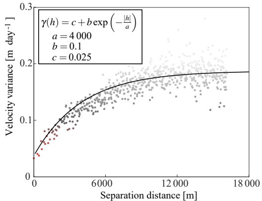
(a) Experimental variogram in the spatial domain
